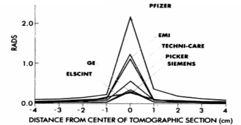
Fig. 7.—Axial dose distributions. Doses were recorded at 1.0 cm intervals from central, single CT section (0 on abscissa) for each CT scanner model. Curves can be used to estimate cumulative dose from series of scans at arbitrary intervals [1].
